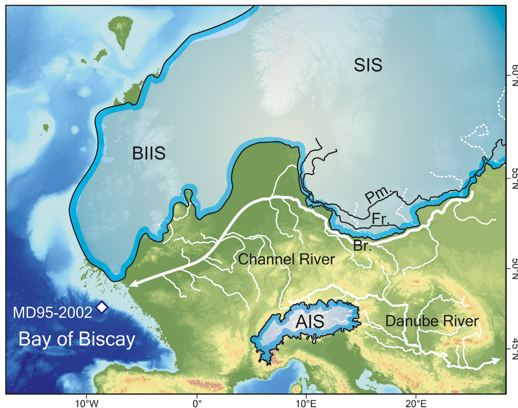
Fig. 2. Palaeogeography of western Europe at the Last Glacial Maximum. The glacial limits of the western European Ice Sheet (EIS), including the Scandinavian (SIS), British-Irish (BIIS) components, and Alpine Ice Sheet (AIS) are shown, along with the Channel and Danube river hydrographic networks (white arrows). Br. Brandenburg-Lesno moraine (formed between 23.4 \pm 0.3 and 20.3 \pm 0.2 ka), Fr. Frankfurt-Poznan moraine (from 18.7 \pm 0.3 to 18.2 \pm 0.2 ka), Pm.: Pomeranian moraine (from 16.7 \pm 0.2 to 15.7 \pm 0.3 ka) (Toucanne et al., 2015). The location of core MD95-2002 in the Bay of Biscay is also shown.
